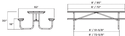
158-GRY6 6' Heavy-Duty Rectangular Table, portable, grey recycled plastic planks, black frame
